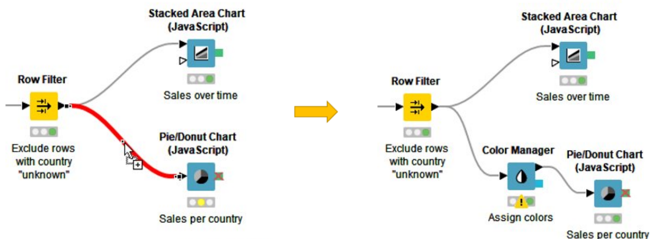
Figure 16. Insert a node between two nodes in a workflow
