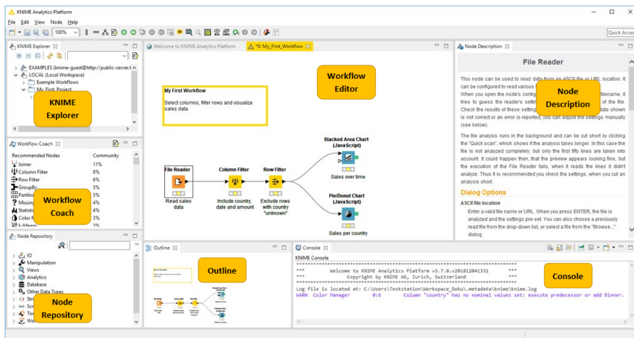
Figure 2. KNIME Workbench
