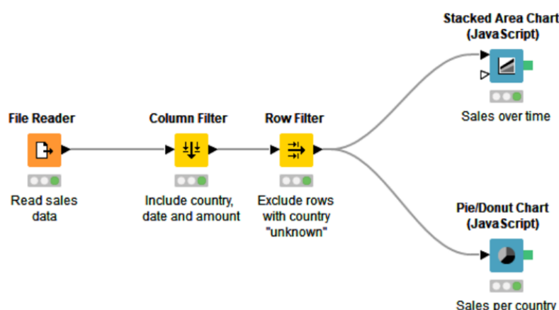
Figure 4. Example workflow
