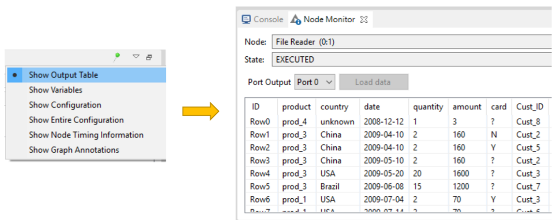
Figure 24. Showing output table in the node monitor
