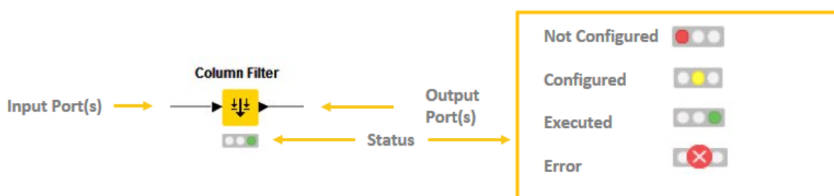
Figure 3. Node ports and node status
