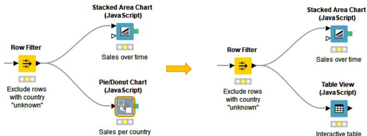
Figure 21. Replacing a node in a workflow
