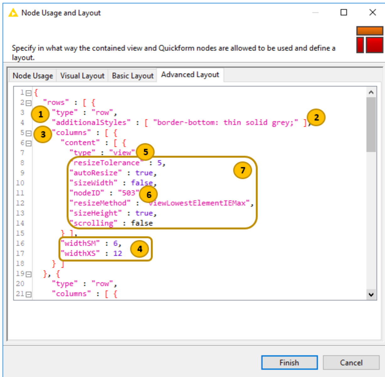
Figure 10. Wrapped Metanode Layouting in JSON Format
