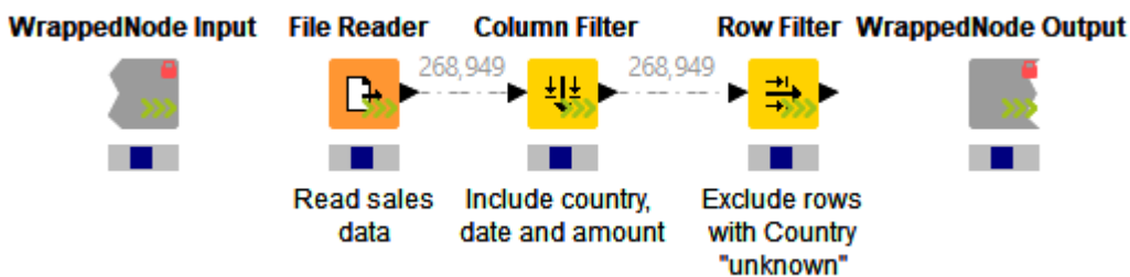
Figure 12. Streaming Execution inside a Wrapped Metanode
