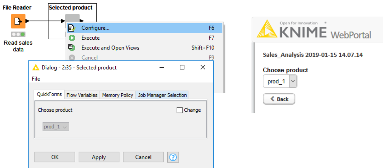
Figure 9. Value Selection Option in the Configuration Dialog of a Wrapped Metanode and on a WebPortal Page
