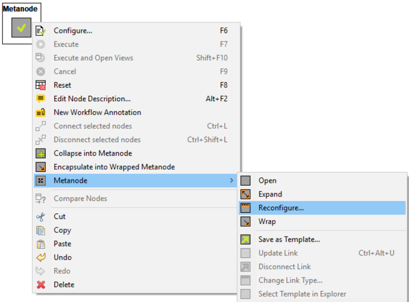
Figure 4. Metanode context menu
