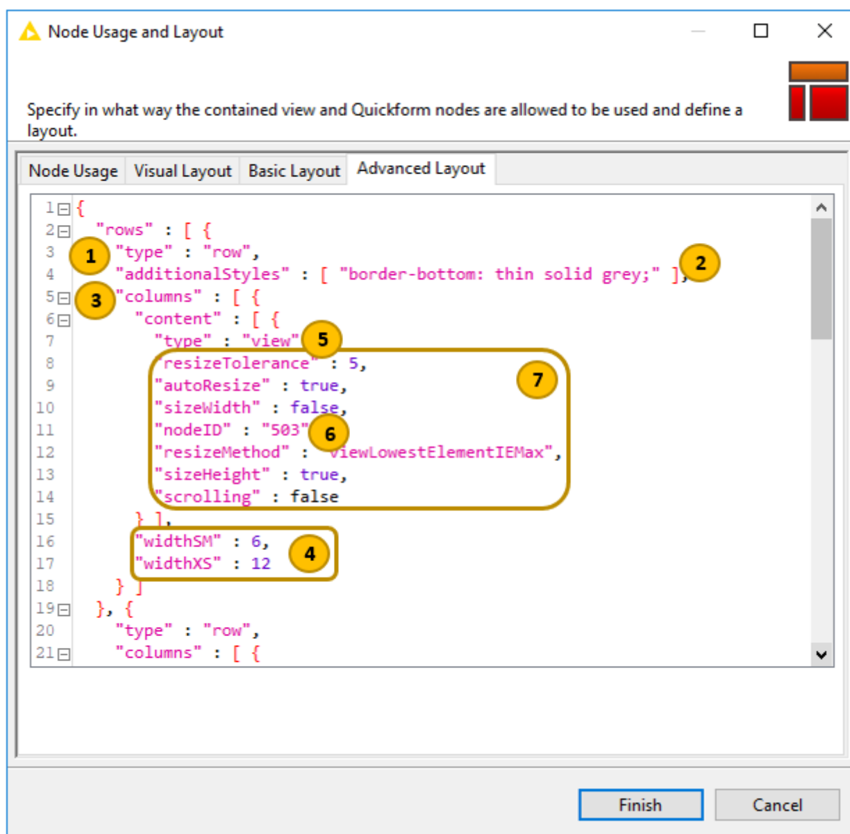
Figure 1. Wrapped Metanode Layouting in JSON Format
