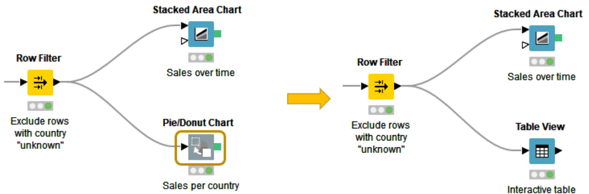
Figure 22. Replacing a node in a workflow
