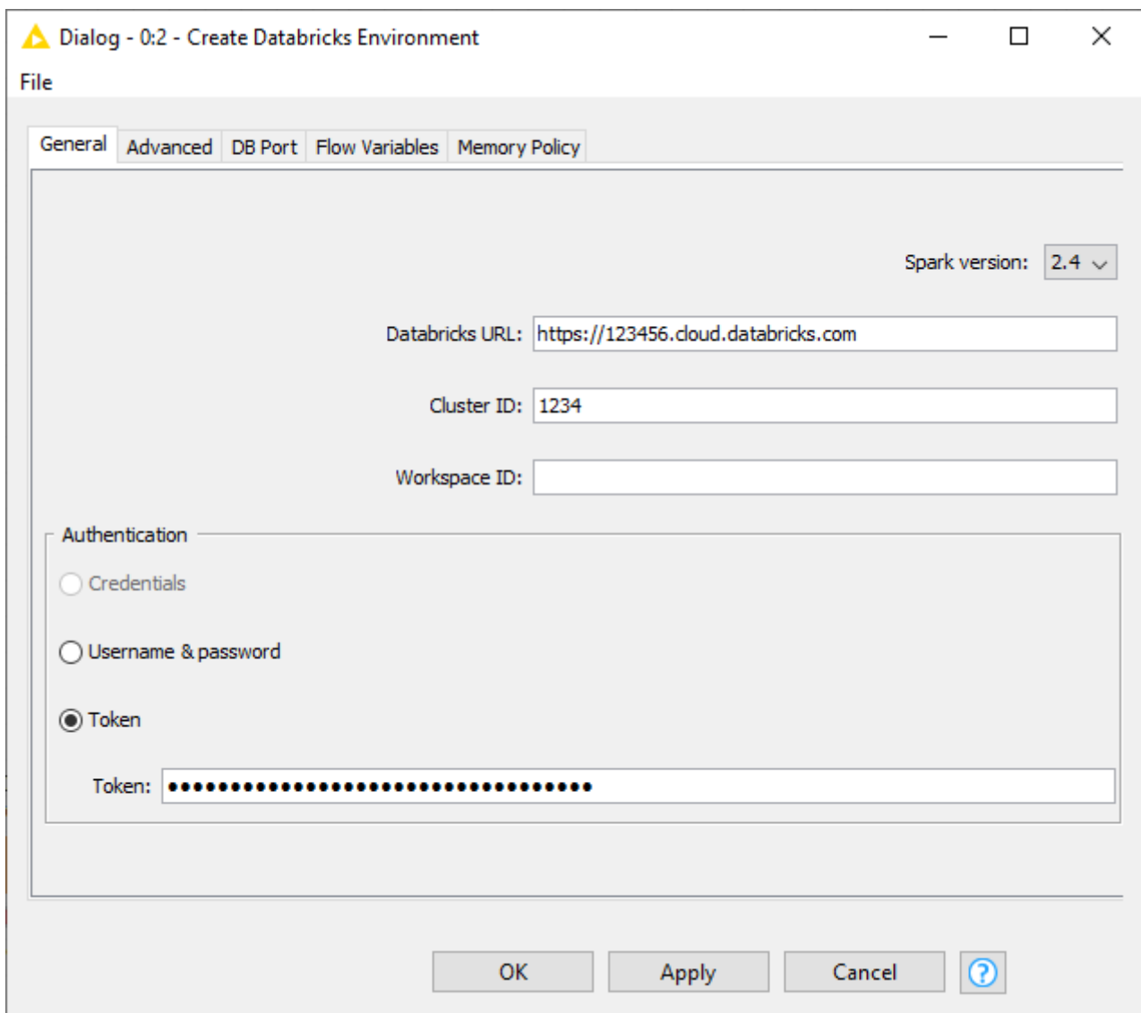
Figure 16. Configuration Window of Create Databricks Environment Node
