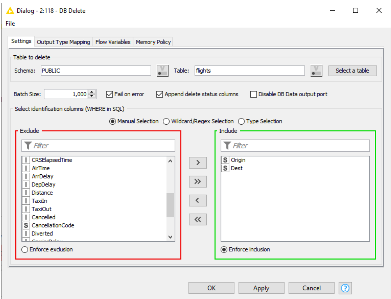
Figure 39. Configuration dialog of the DB Delete node
