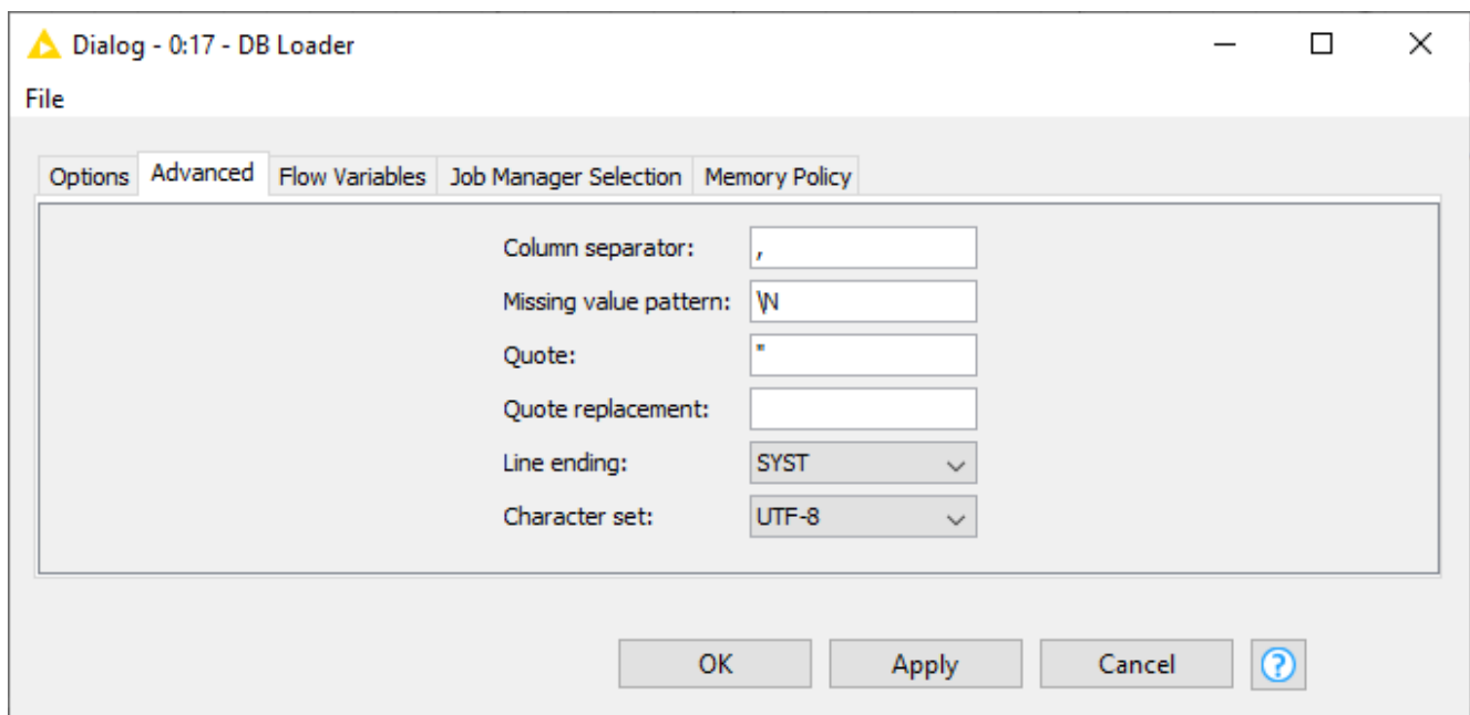
Figure 41. DB Loader: Advanced
