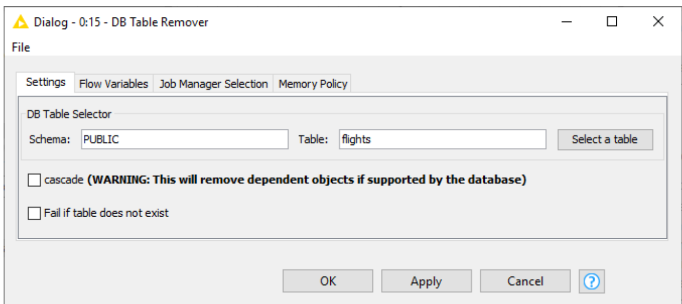
Figure 35. DB Table Remover configuration dialog
