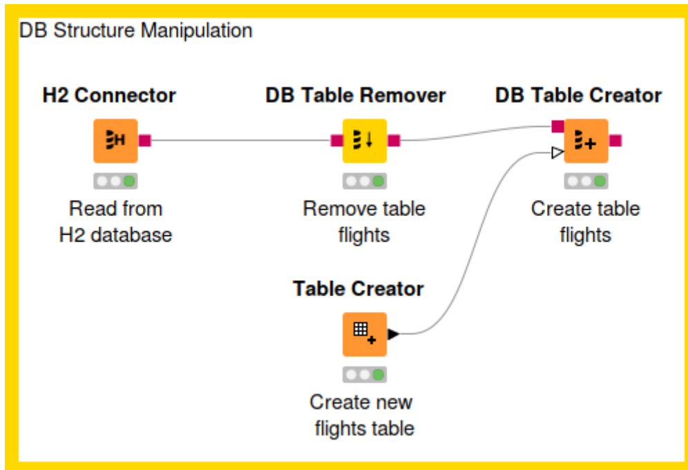
Figure 34. Example of a database structure manipulation workflow
