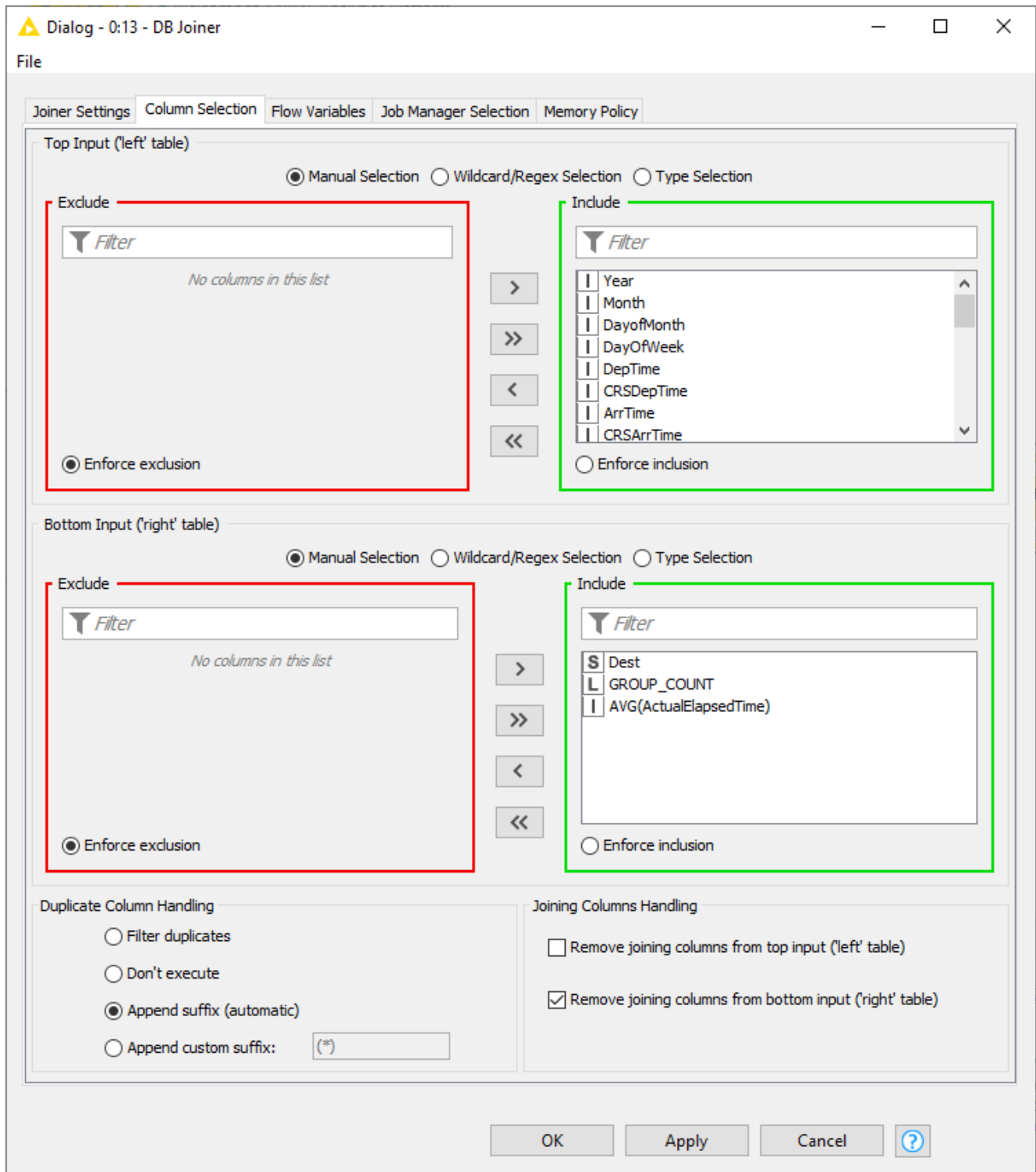
Figure 31. DB Joiner: Column Selection
