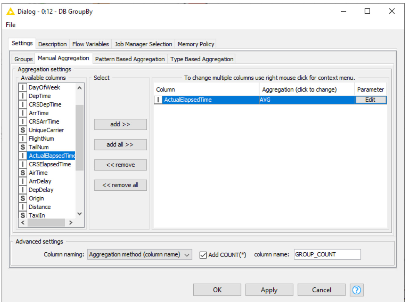
Figure 28. DB GroupBy: Manual Aggregation
