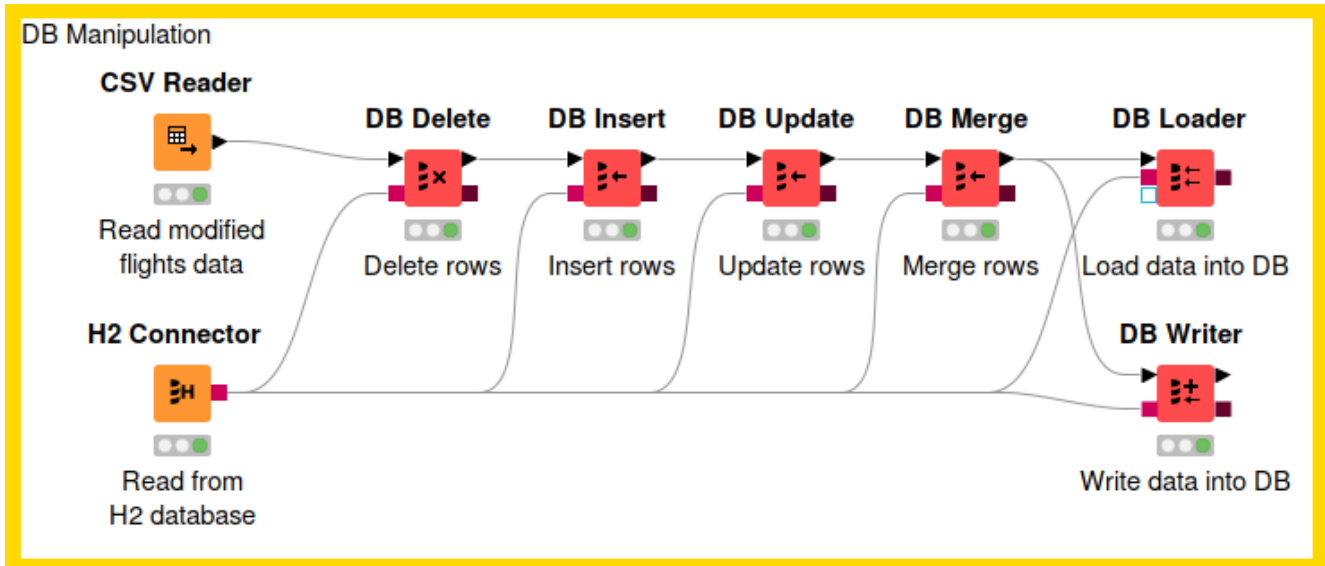
Figure 38. Example of DB Manipulation
