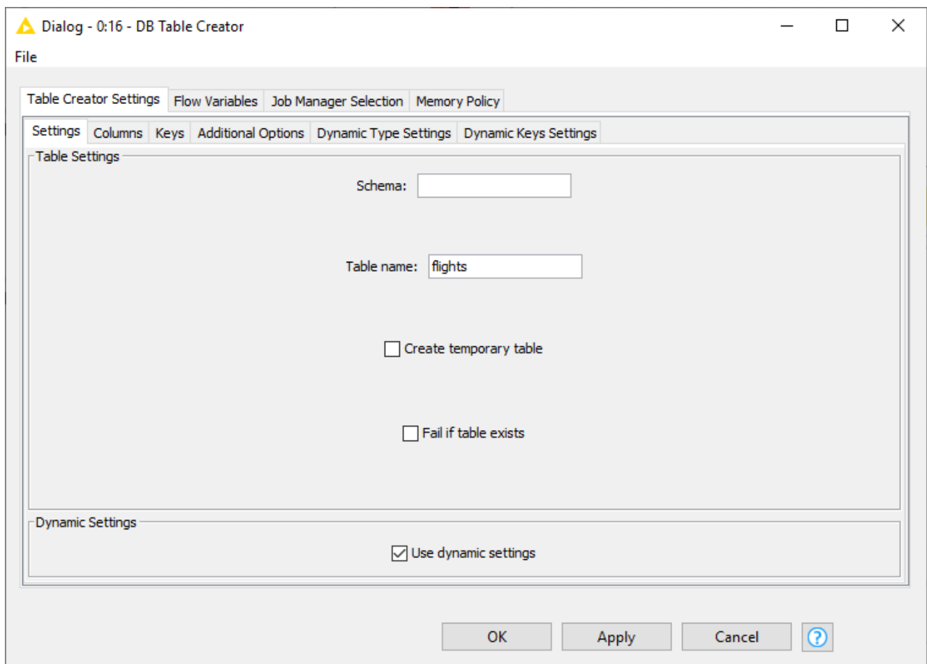
Figure 36. DB Table Creator: Settings
