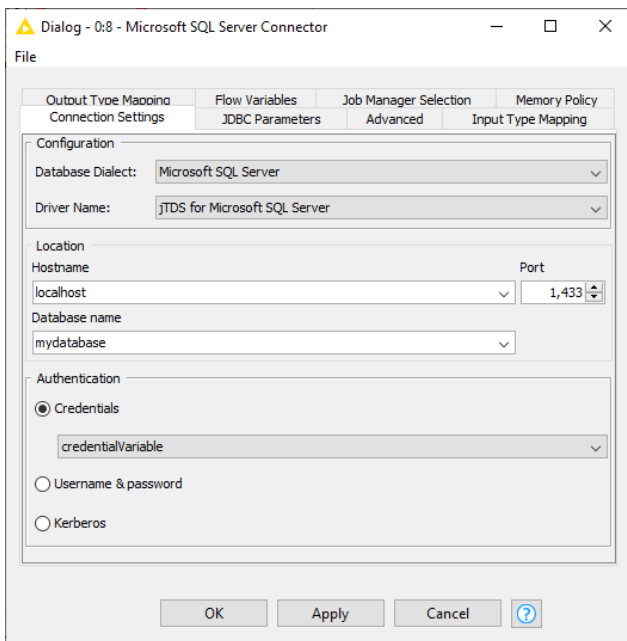
Figure 5. MS SQL Server Connector configuration dialog
