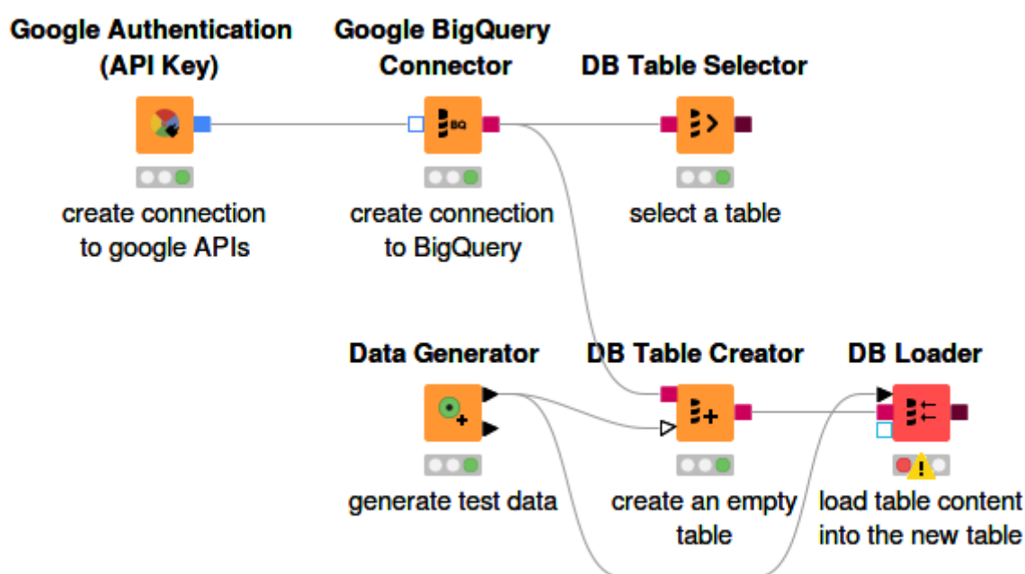
Figure 14. Connecting to and working with Google BigQuery
