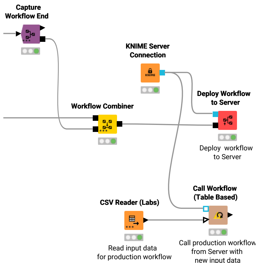
Figure 16. An example workflow to execute the captured workflow from KNIME Server with some input data
