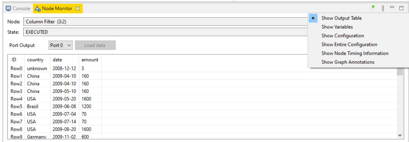
Figure 29. Node Monitor
