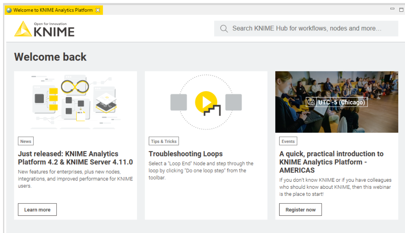
Figure 3. Welcome page
