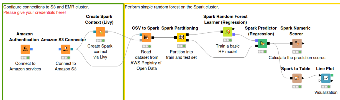
Figure 10. Train a machine learning model on a Spark EMR cluster
