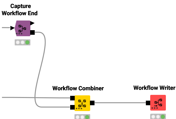
Figure 9. An example workflow to write a captured workflow to the local file system
