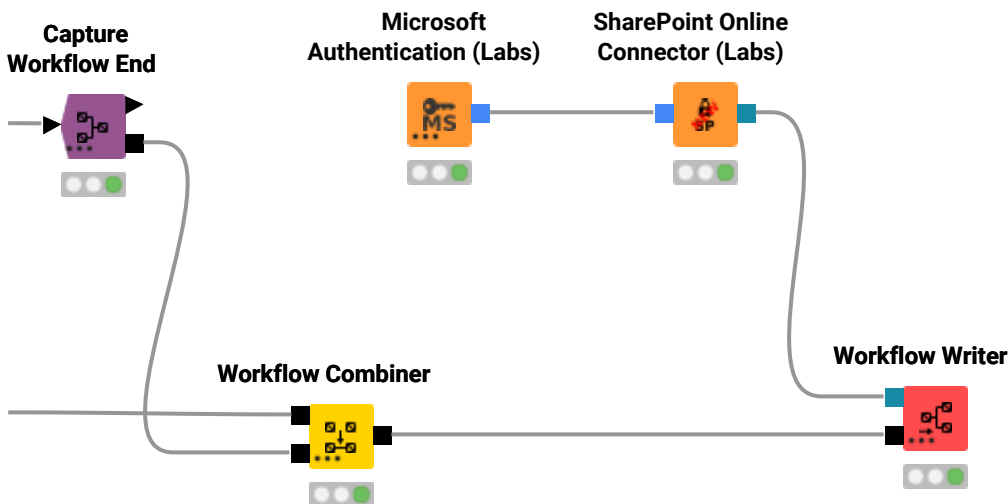
Figure 12. An example workflow to write a captured workflow to a remote file system
