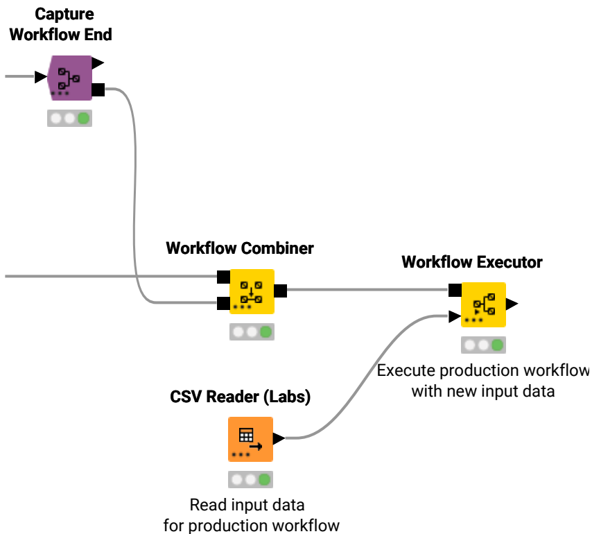
Figure 17. An example workflow to execute the captured workflow locally
