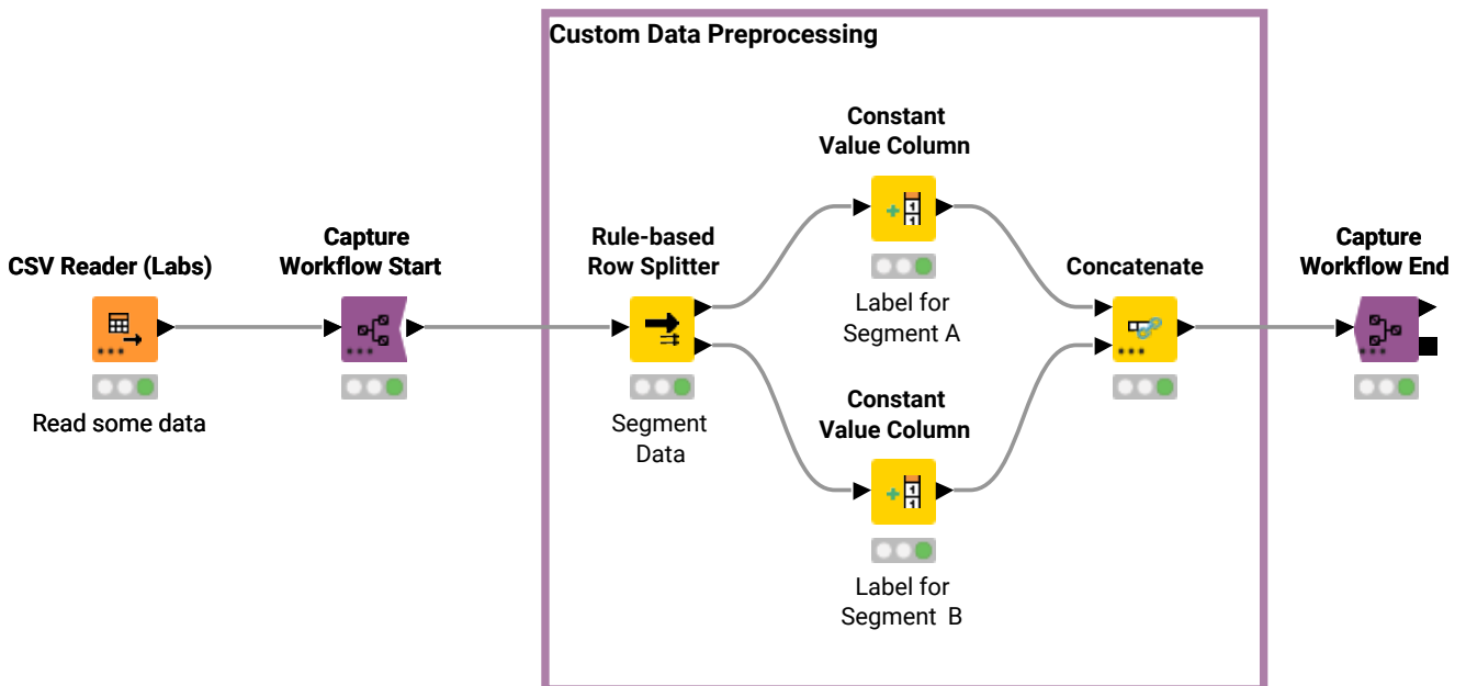
Figure 2. A fragment of a workflow is captured
