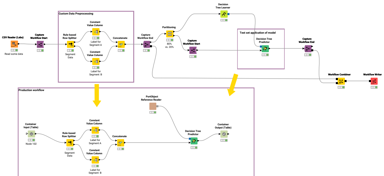
Figure 7. Different fragments of a workflow are captured and combined in a new workflow
