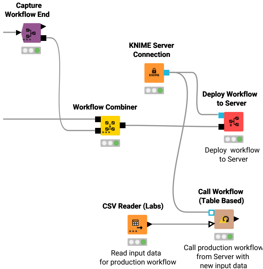
Figure 16. An example workflow to execute the captured workflow from KNIME Server with some input data
