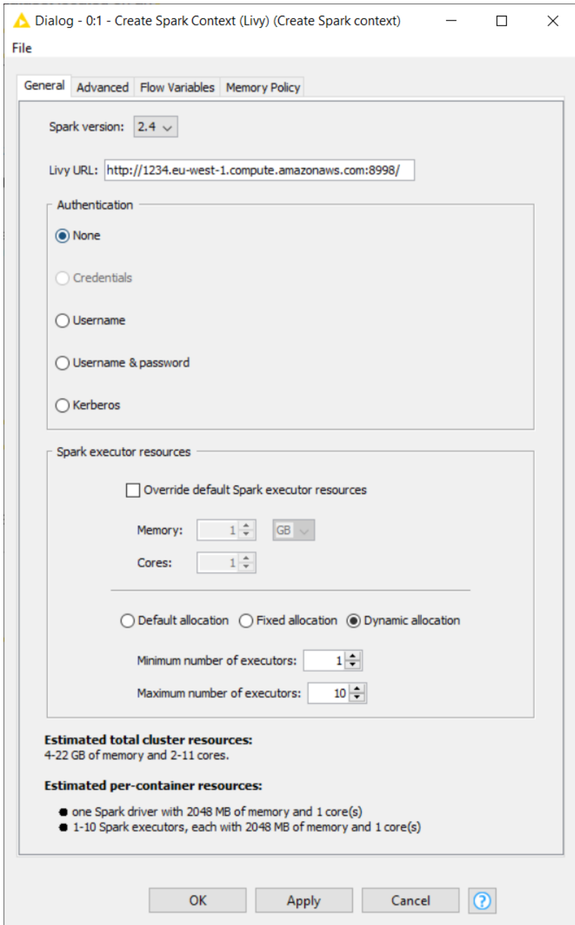
Figure 9. Create Spark Context (Livy) node
