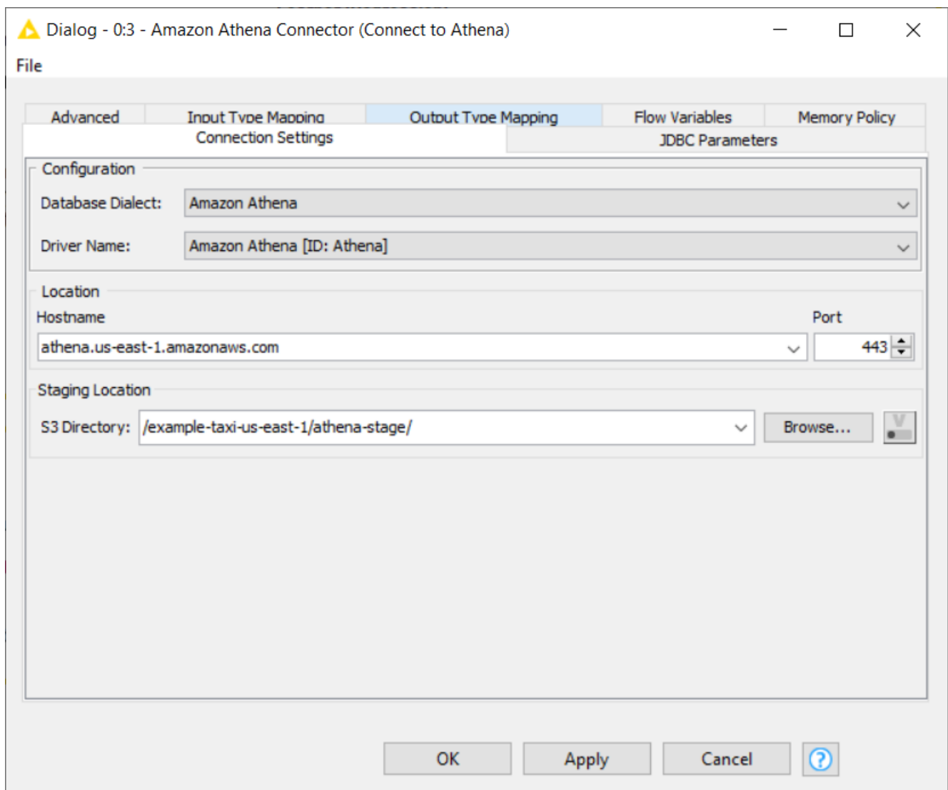
Figure 14. Athena Connector node
