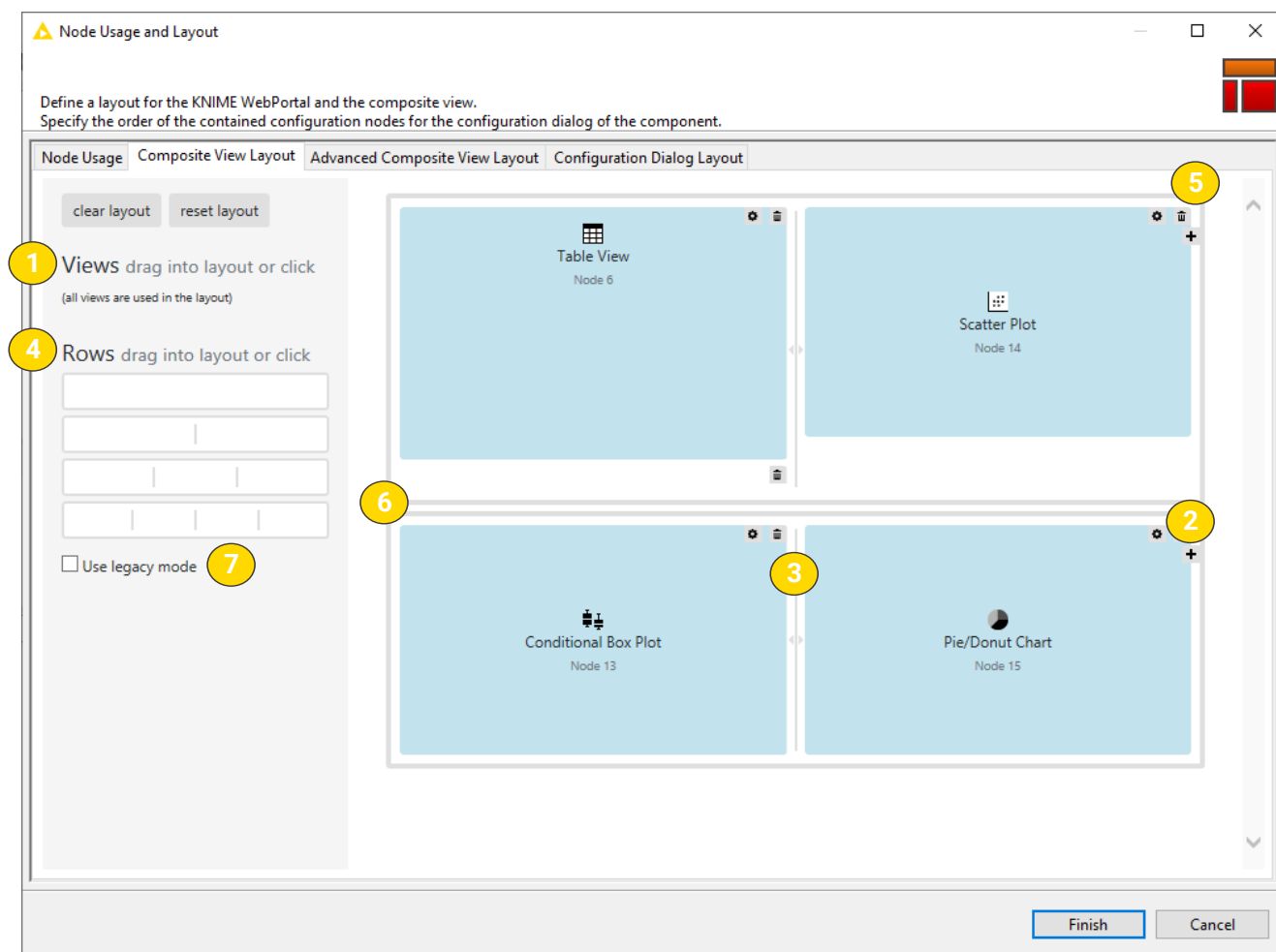
Figure 29. The visual layout editor of a component
