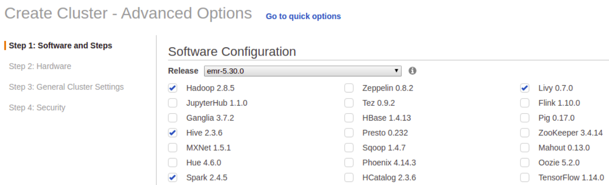
Figure 3. Software configuration
