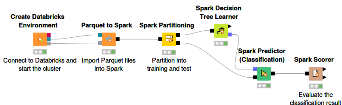
Figure 16. Example of machine learning application using Spark nodes on Databricks
