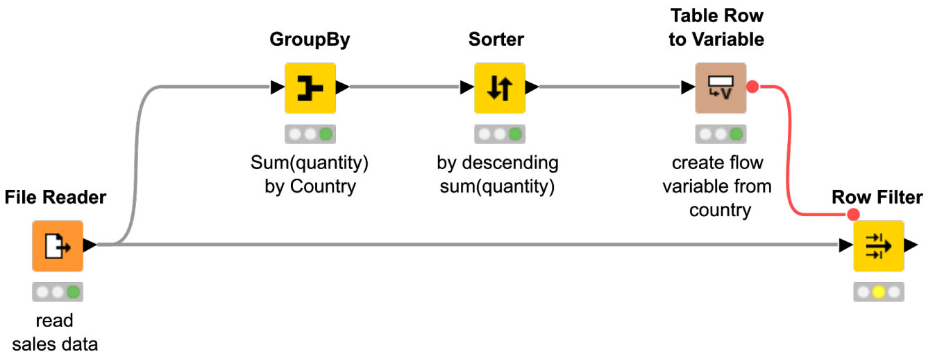
Figure 2. Converting first row of a data table to flow variables
