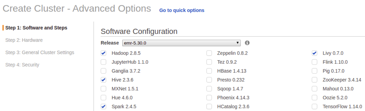
Figure 3. Software configuration
