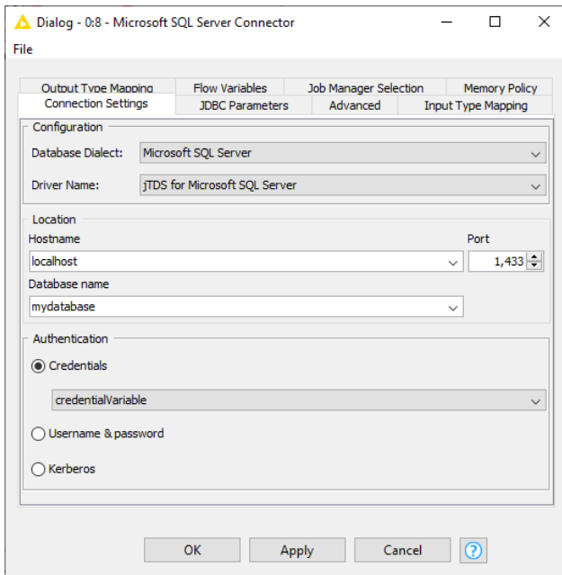
Figure 5. MS SQL Server Connector configuration dialog
