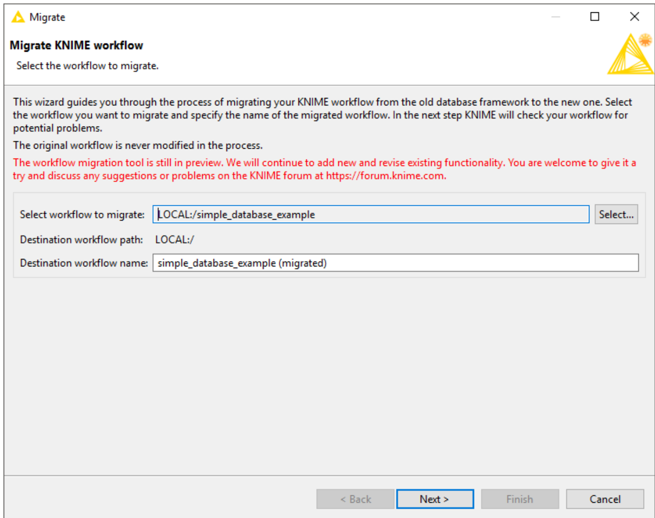
Figure 52. Migration Tool: Select the workflow
