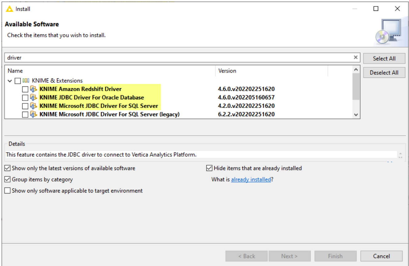
Figure 6. Install Window
