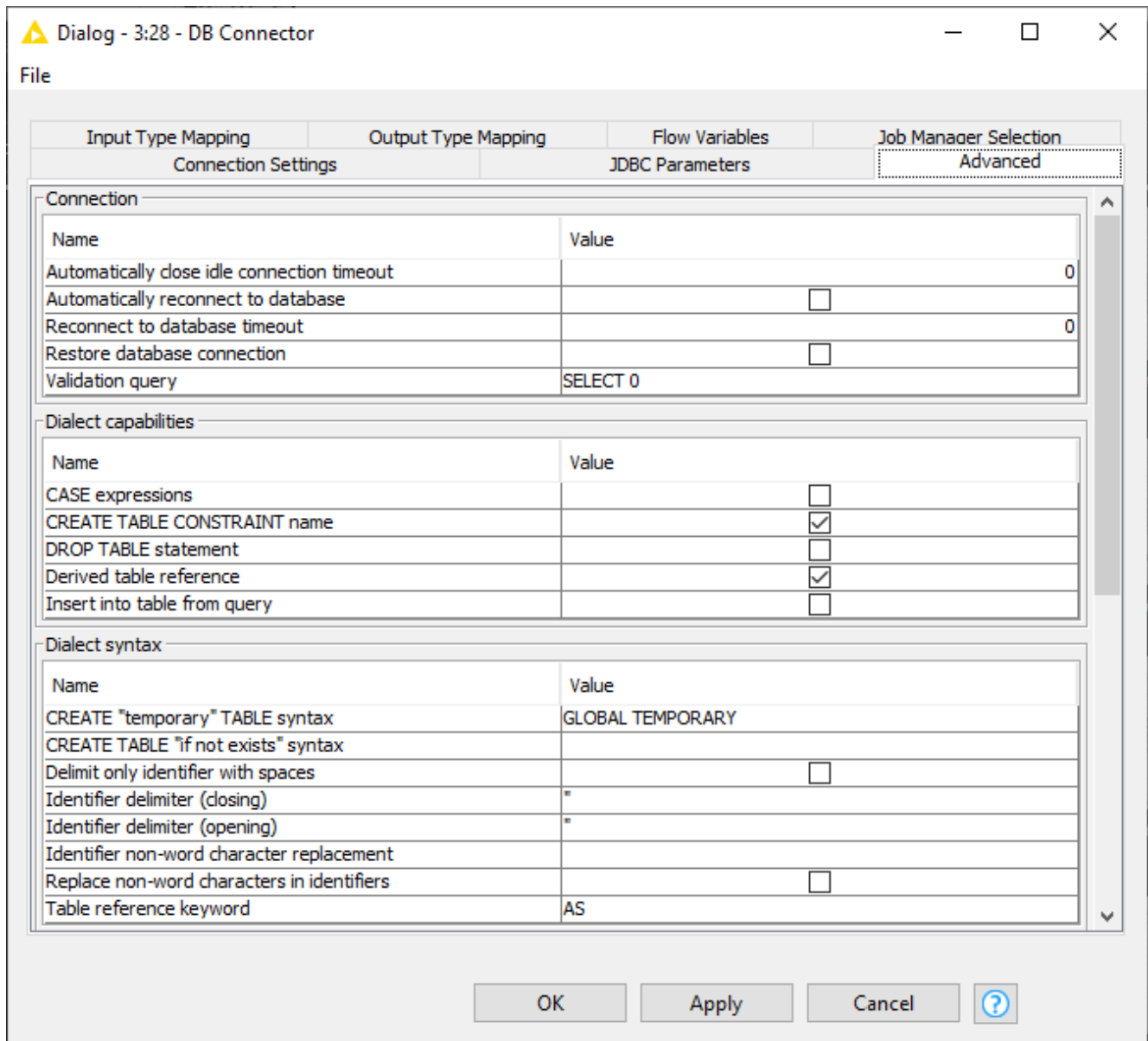
Figure 11. Advanced Tab
