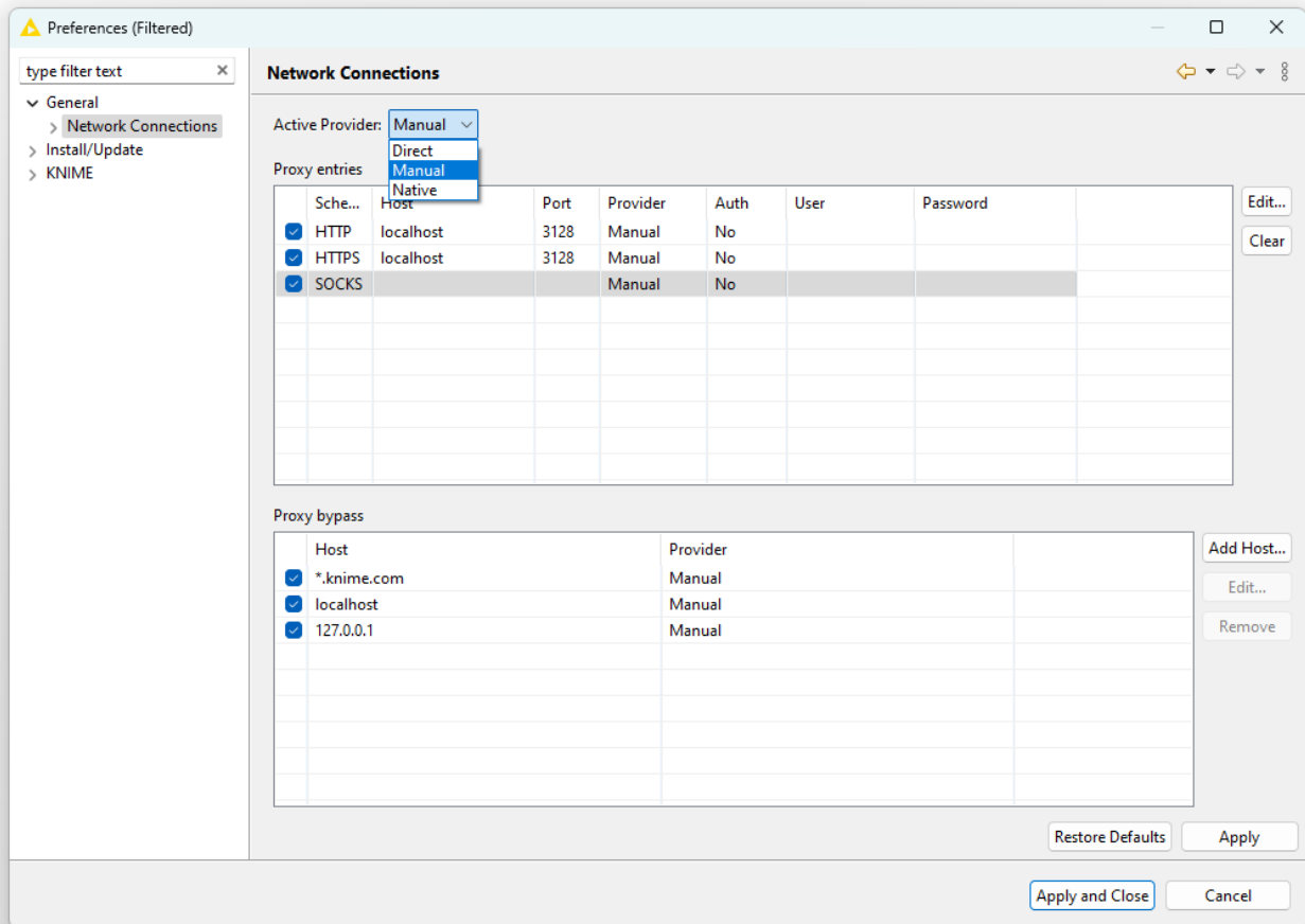
Figure 32. The Network Connections preferences page
