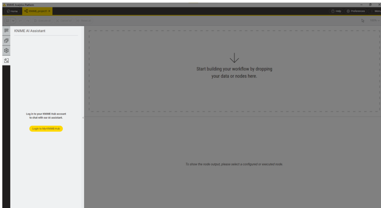
Figure 23. Login
