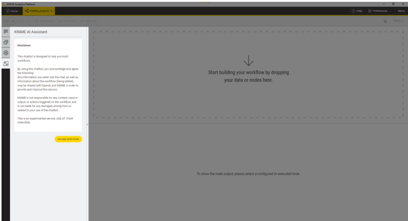
Figure 25. Disclaimer
