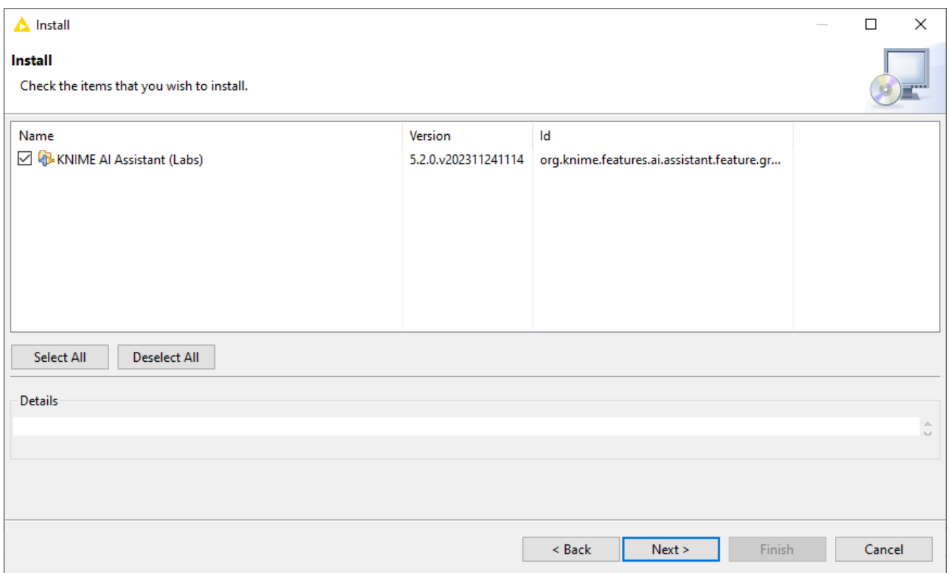
Figure 22. Installation menu
