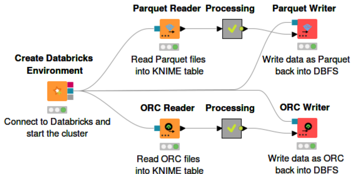
Figure 9. Parquet/ORC Reader and Writer nodes
