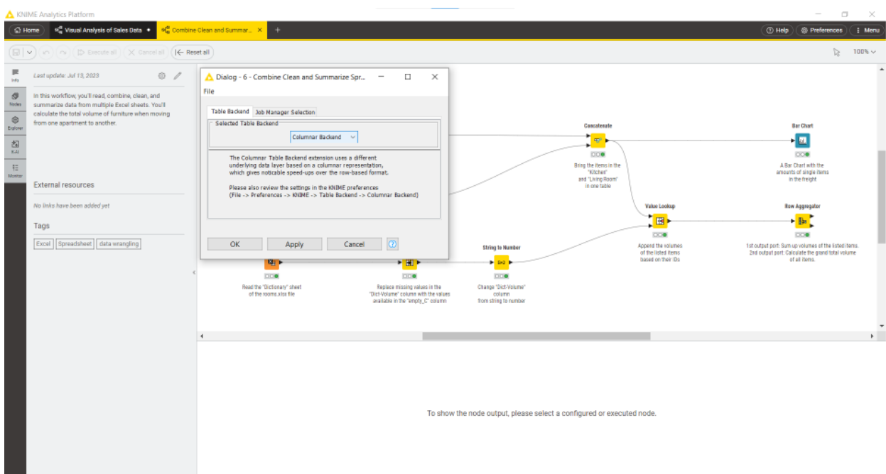
Figure 30. Configure a workflow to use Columnar Backend
