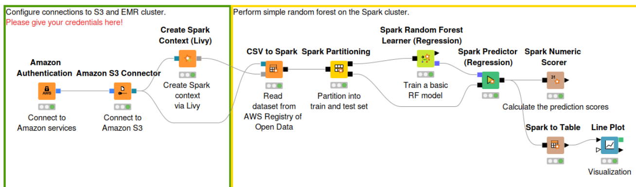
Figure 14. Train a machine learning model on a Spark EMR cluster
