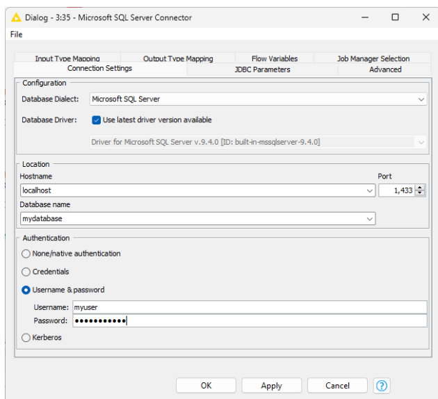
Figure 5. MS SQL Server Connector configuration dialog
