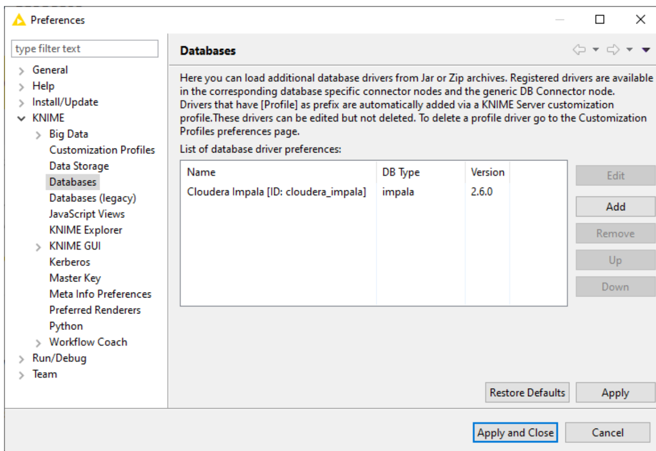
Figure 30. Database Preference page
