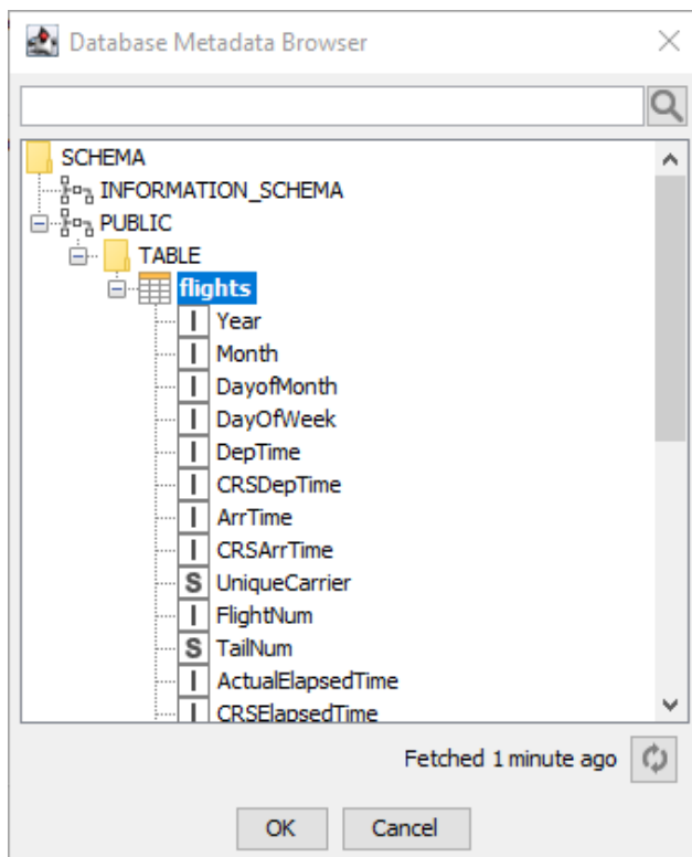
Figure 33. Database Metadata Browser
