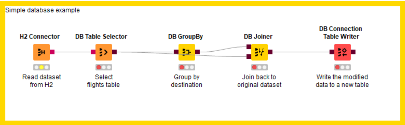
Figure 58. New workflow containing migrated DB nodes
