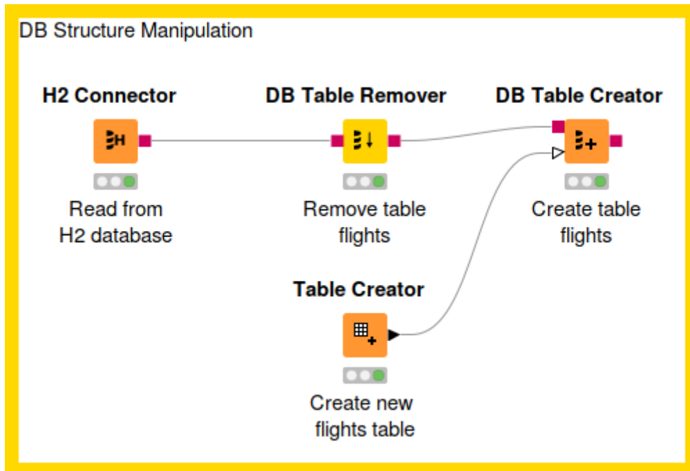
Figure 43. Example of a database structure manipulation workflow
