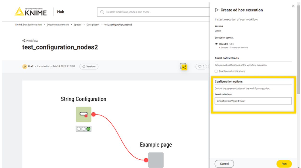
Figure 34. Workflow parameters set in the execution side panel
