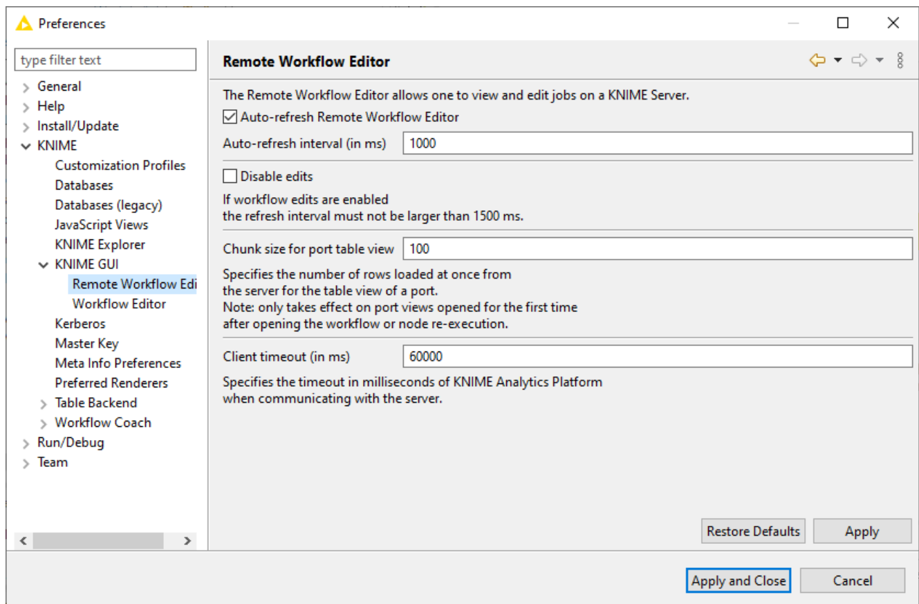
Figure 20. The Remote Workflow Editor preferences window
