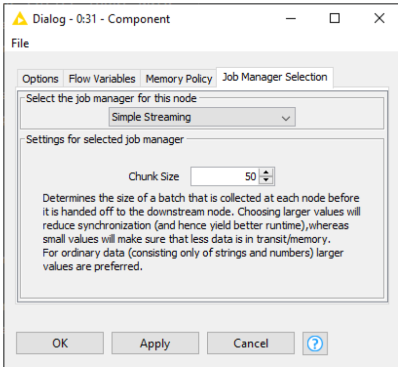
Figure 30. Streaming execution mode and chunk size selection
