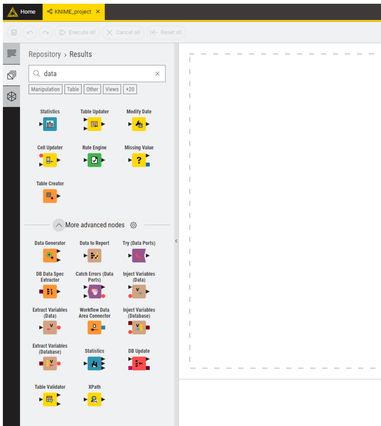
Figure 18. Node repository with two search modes
