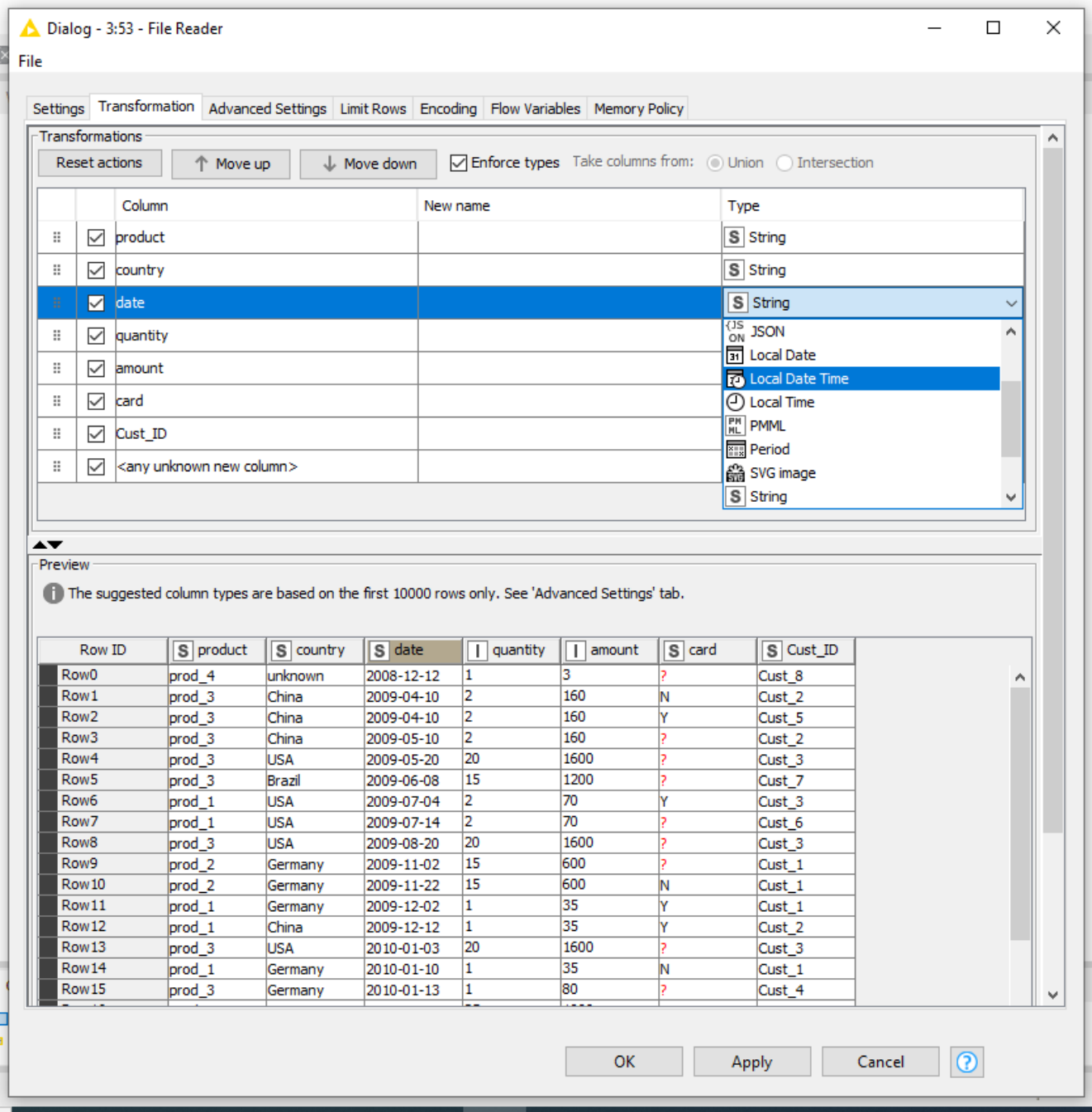
Figure 39. Change column type in File Reader node
