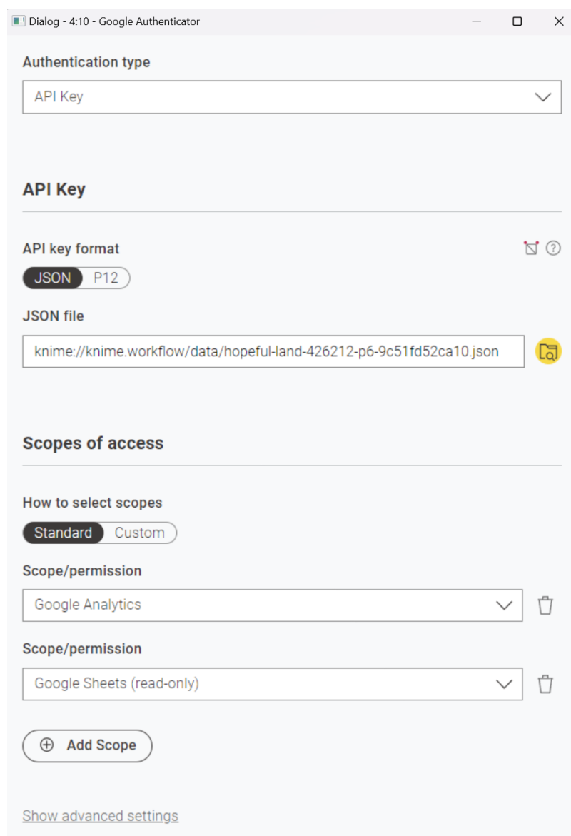
Figure 38. Configuration dialog of Google Authenticator for workflow data area path
