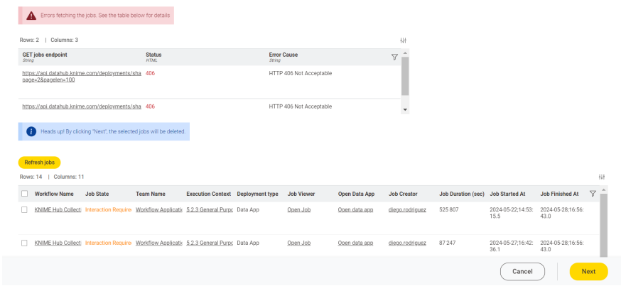
Figure 46. GET Request error displayed in the data app
