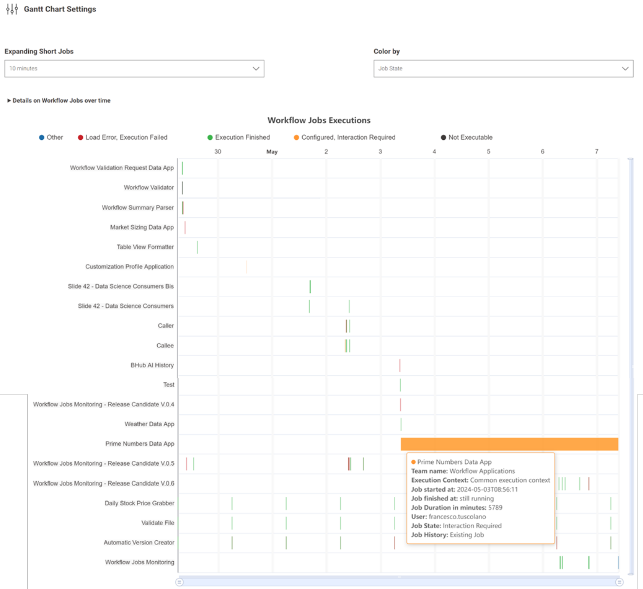
Figure 59. Gantt Chart Settings section of the Workflows Jobs Monitoring data app
