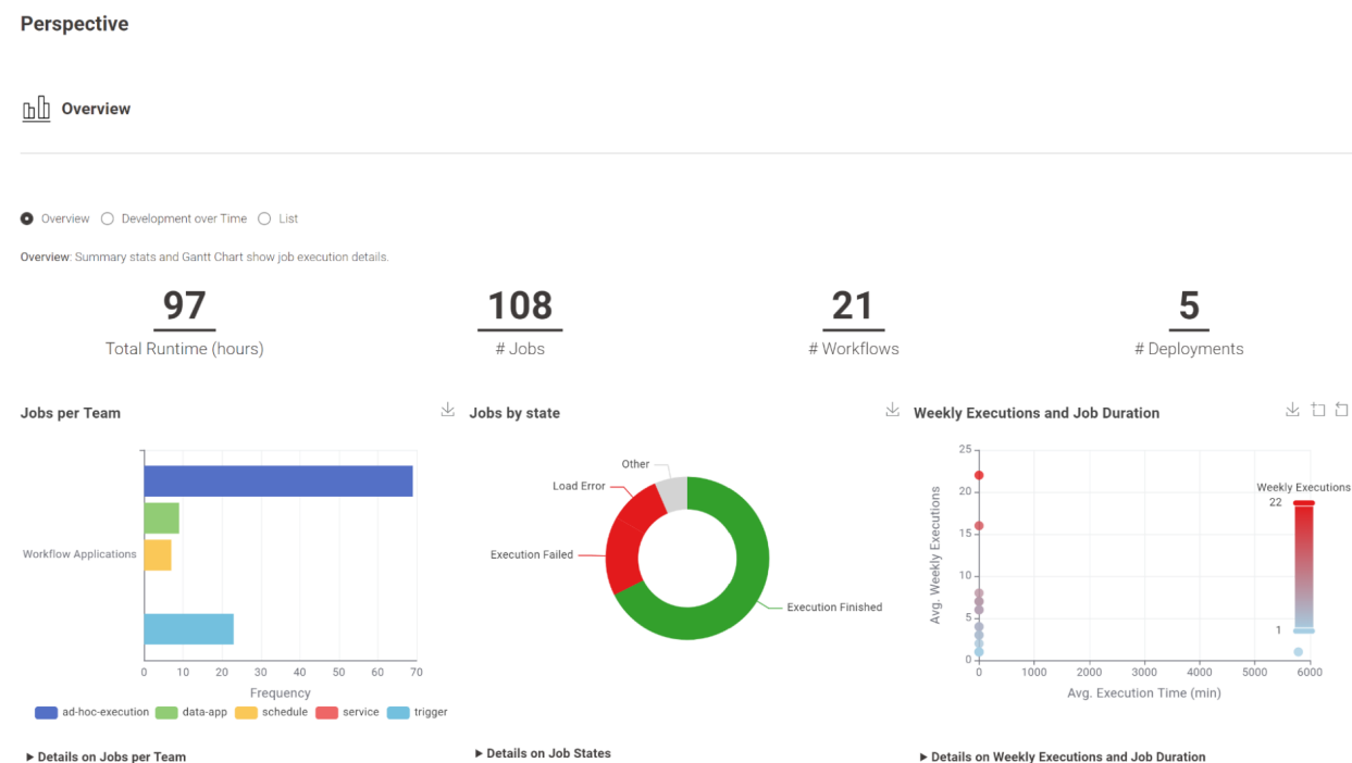
Figure 58. Overview section of the Workflows Jobs Monitoring data app
