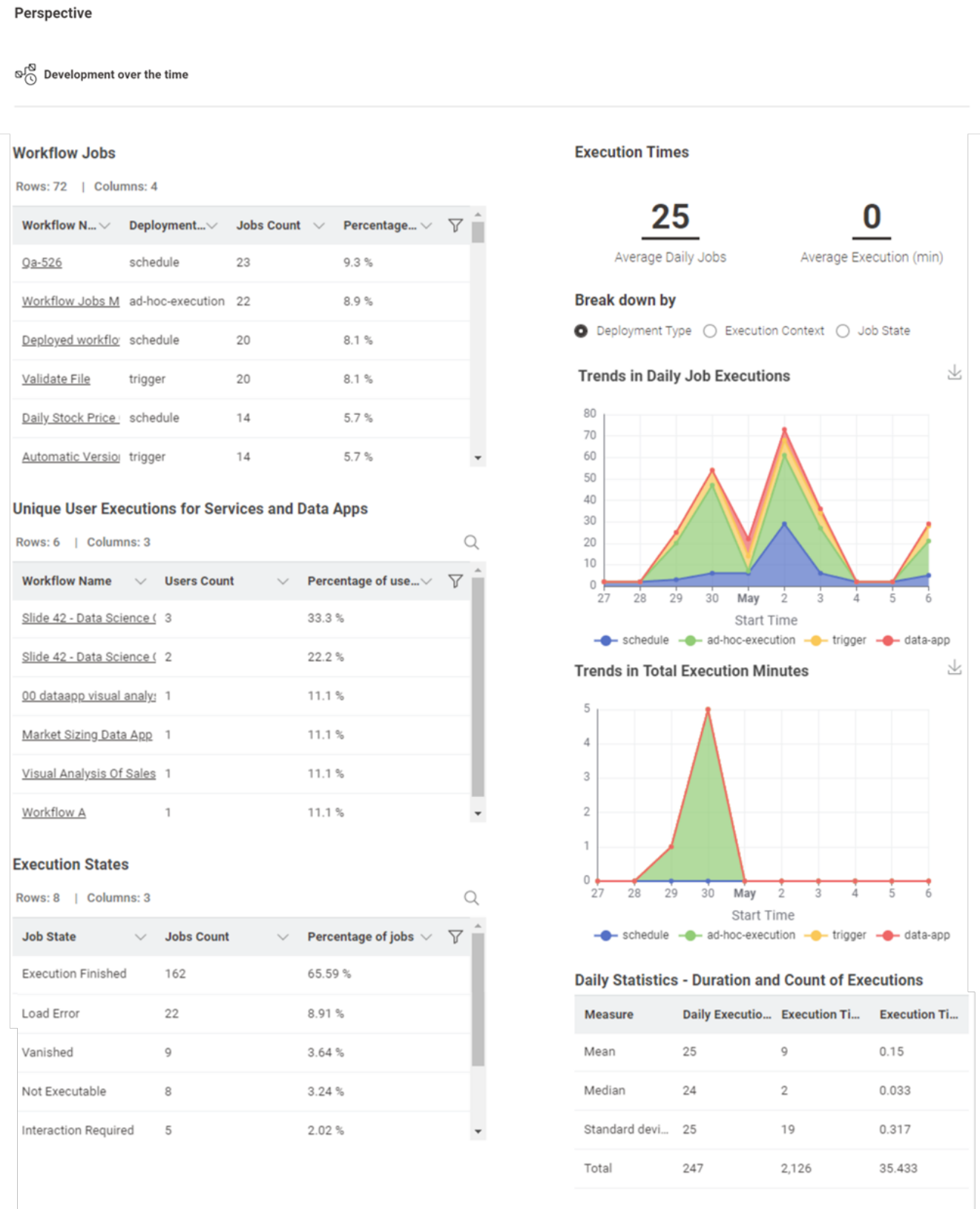
Figure 60. Development over the time section of the Workflows Jobs Monitoring data app
